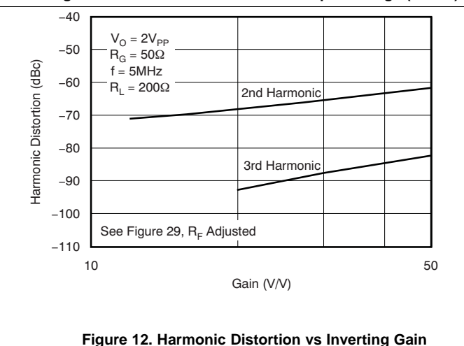
Figure 12. Harmonic Distortion vs Inverting Gain
