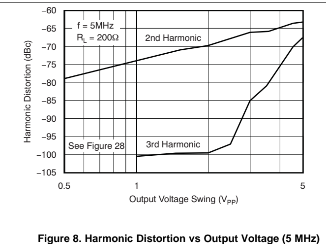
Figure 8. Harmonic Distortion vs Output Voltage (5 MHz)
