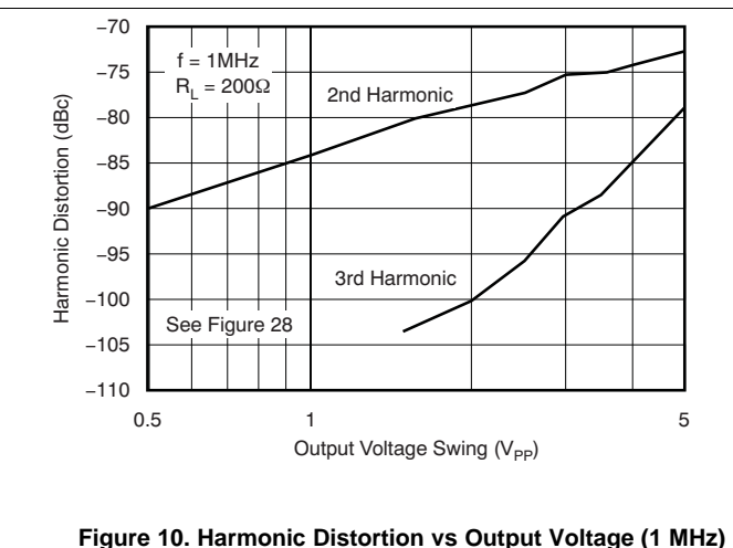
Figure 10. Harmonic Distortion vs Output Voltage (1 MHz)
