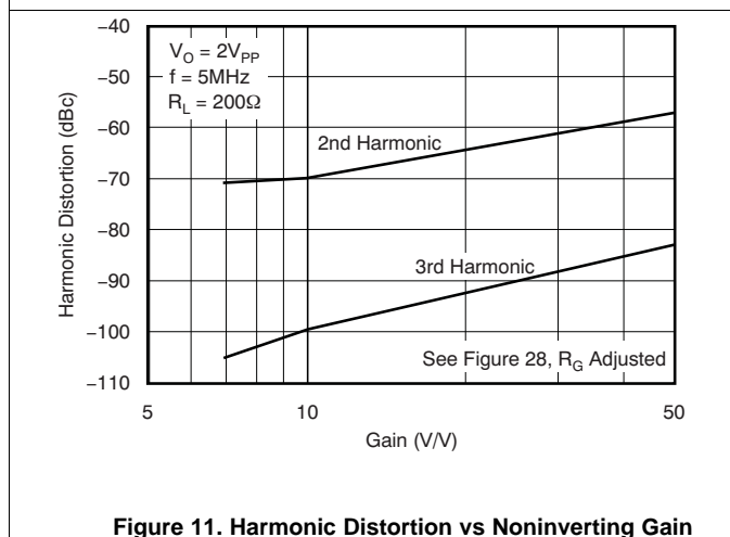
Figure 11. Harmonic Distortion vs Noninverting Gain
